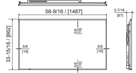
Screw holes for mounting brackets *1,2 Unit: inch [mm]
