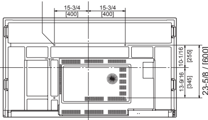
Screw holes for mounting brackets *1,2 Unit: inch [mm]
